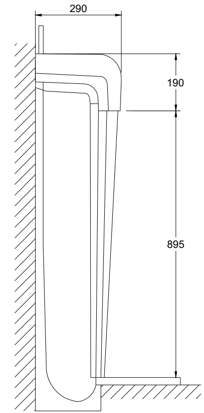
Section BB
